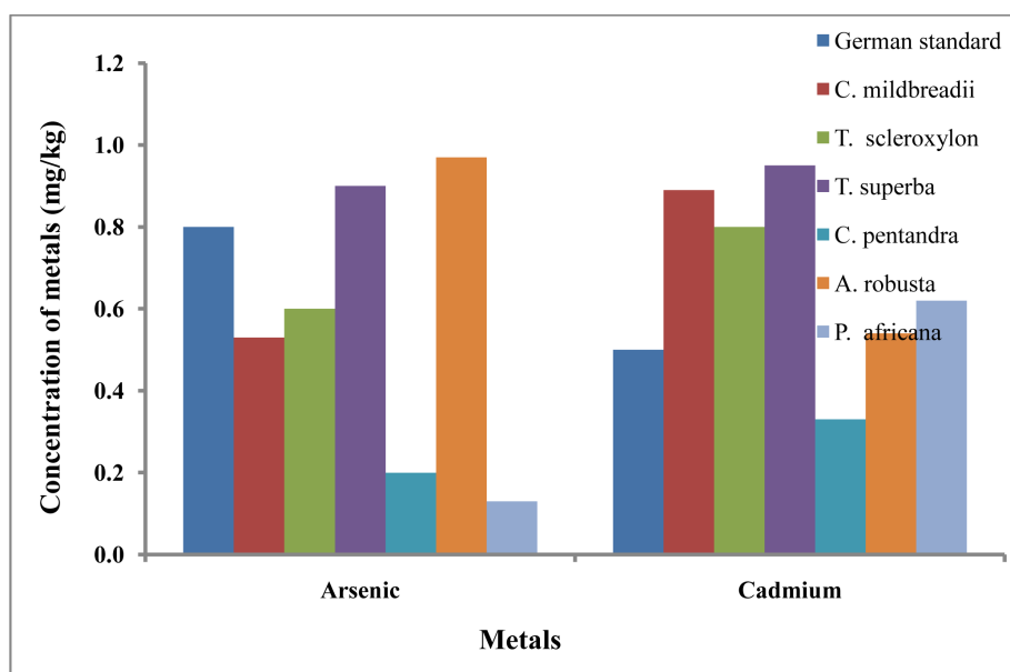
Figure 2. Concentration of arsenic and cadmium in sawdust of six tropical hardwood species.
