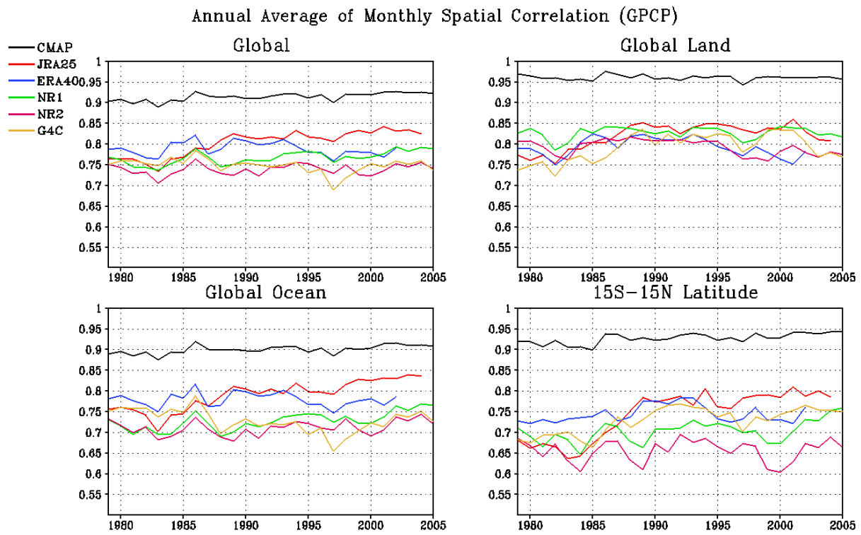
Figure 2 Annual average of monthly spatial correlations to GPCP for global areas.
