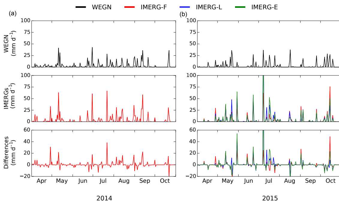
Figure 3. Accumulated 24 h rainfall ( \text{mm day}^{-1} ) over the study periods in 2014 (a) and 2015 (b), obtained from WEGN (top) and IMERG runs (middle), and differences between IMERG and WEGN (bottom). Regarding IMERG in the 2014 period, only IMERG-F data are available.
