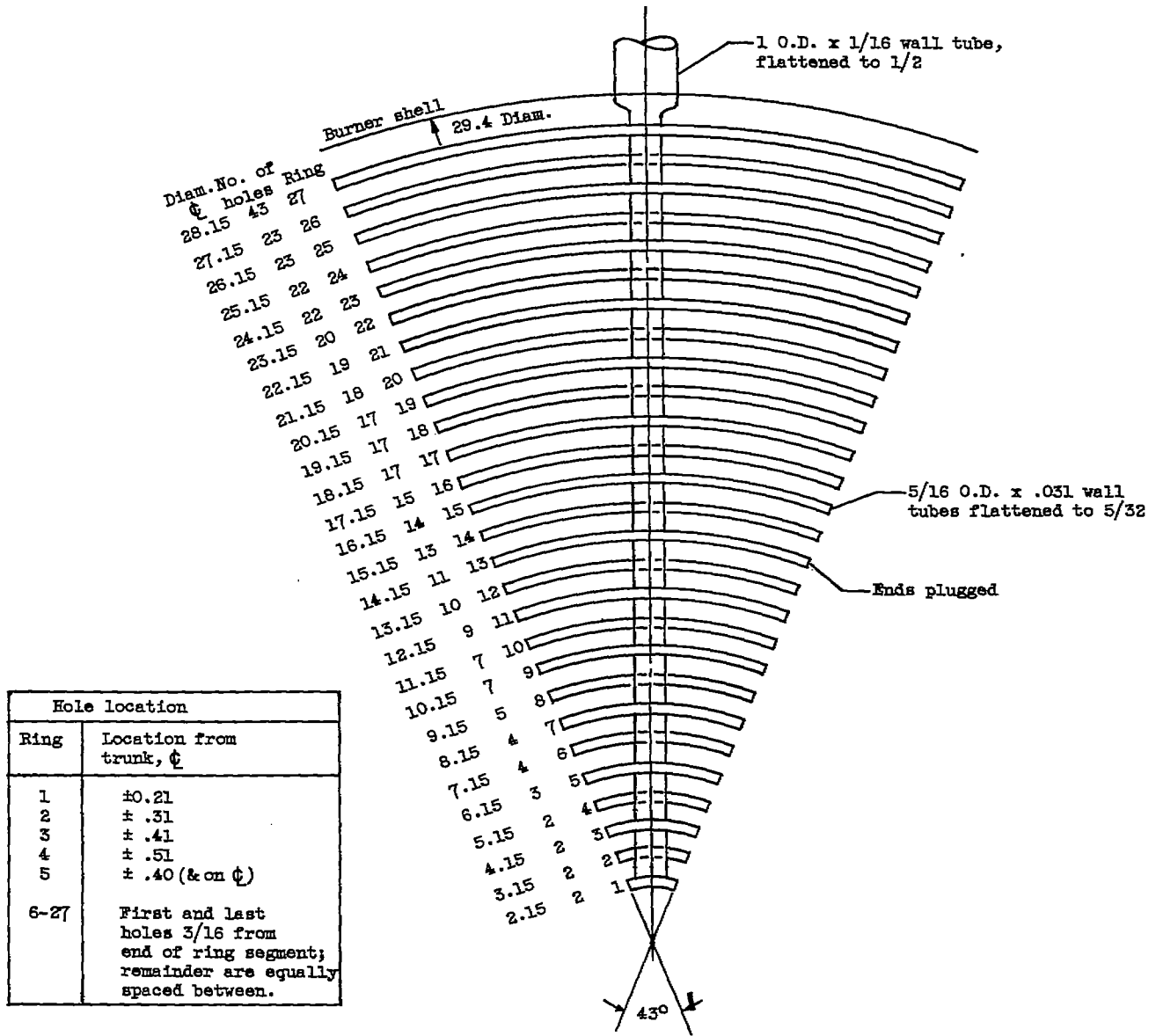
Figure 7. - Fuel-injector sector, configuration B; 8 sectors required. Material, Inconel; all holes, 0.026-inch diameter; all holes drilled for 100-percent axial injection. Total number of holes, 351. (All dimensions in inches.)
