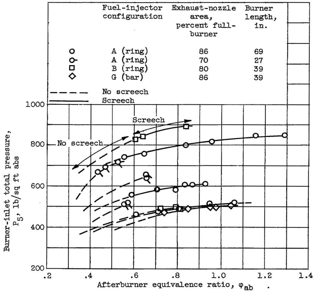
Figure 20. - Occurrence of audible screech at steady-state operating conditions as noted for all configurations investigated. (Data points represent operation in screech.)
