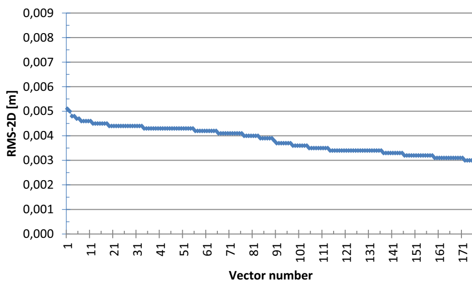
Fig. 6. RMS-2D for common vectors of ASG-EUPOS and GeoTerrace networks, GPS Week Number 19064.
