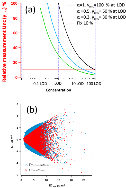
Figure 1. (a) Example \gamma_{unc} -nonlinear curves by different \alpha values (Eq. 17). The x axis is concentration (normalized by LOD) in log scale and the y axis is \gamma_{unc} . Black, blue and green line represents \alpha equal to 1, 0.5 and 0.3, respectively, corresponding to the \gamma_{unc} -nonlinear at LOD level equals to 100, 50 and 30 %, respectively. The red line represents \gamma_{unc} -linear of 10 %. (b) Example of measurement uncertainty generation of \gamma_{unc} -nonlinear and \gamma_{unc} -linear. The blue circles represent \gamma_{unc} -nonlinear following Eq. (17) ( LOD_{EC} = 1, a_{EC} = 1 ). The red circles represent \gamma_{unc} -linear (30 %).
