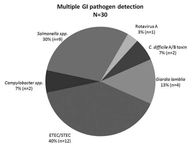
FIG 1 Targets detected in coinfections. GPP ASRs detect multiple GI pathogens undetected in clinical specimens by conventional methods, indicating the potential for multiplex technology in the identification of coinfection in patient stools. The percentage of incidence indicates the most predominant ADD targets detected in single specimens. ETEC and STEC were the most predominant strains detected followed by Salmonella spp. and Giardia lamblia .
