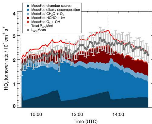
Figure 4. \text{HO}_2 budget for the MBO experiment. The loss rate of \text{HO}_2 calculated from measured NO, ozone, and \text{HO}_2 concentrations, L_{\text{HO}_2\text{Meas}} , and individual modelled production terms are shown. For comparison, the red line indicates the total modelled \text{HO}_2 production, P_{\text{HO}_2\text{Mod}} , which equals the total modelled loss rate. Vertical dashed lines indicate the times when MBO was injected. Error bars ( 1\sigma ) for L_{\text{HO}_2\text{Meas}} include the accuracy of \text{HO}_2 measurements.
