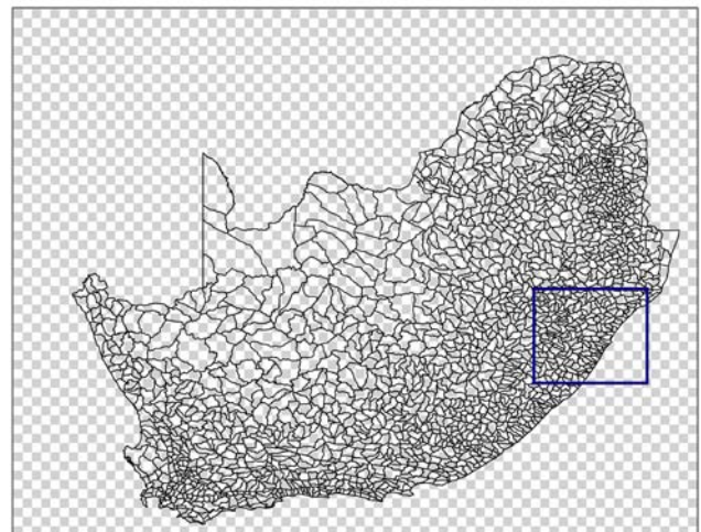
Figure 1 An 0.25^\circ resolution grid overlaid by the quaternary catchment boundaries
