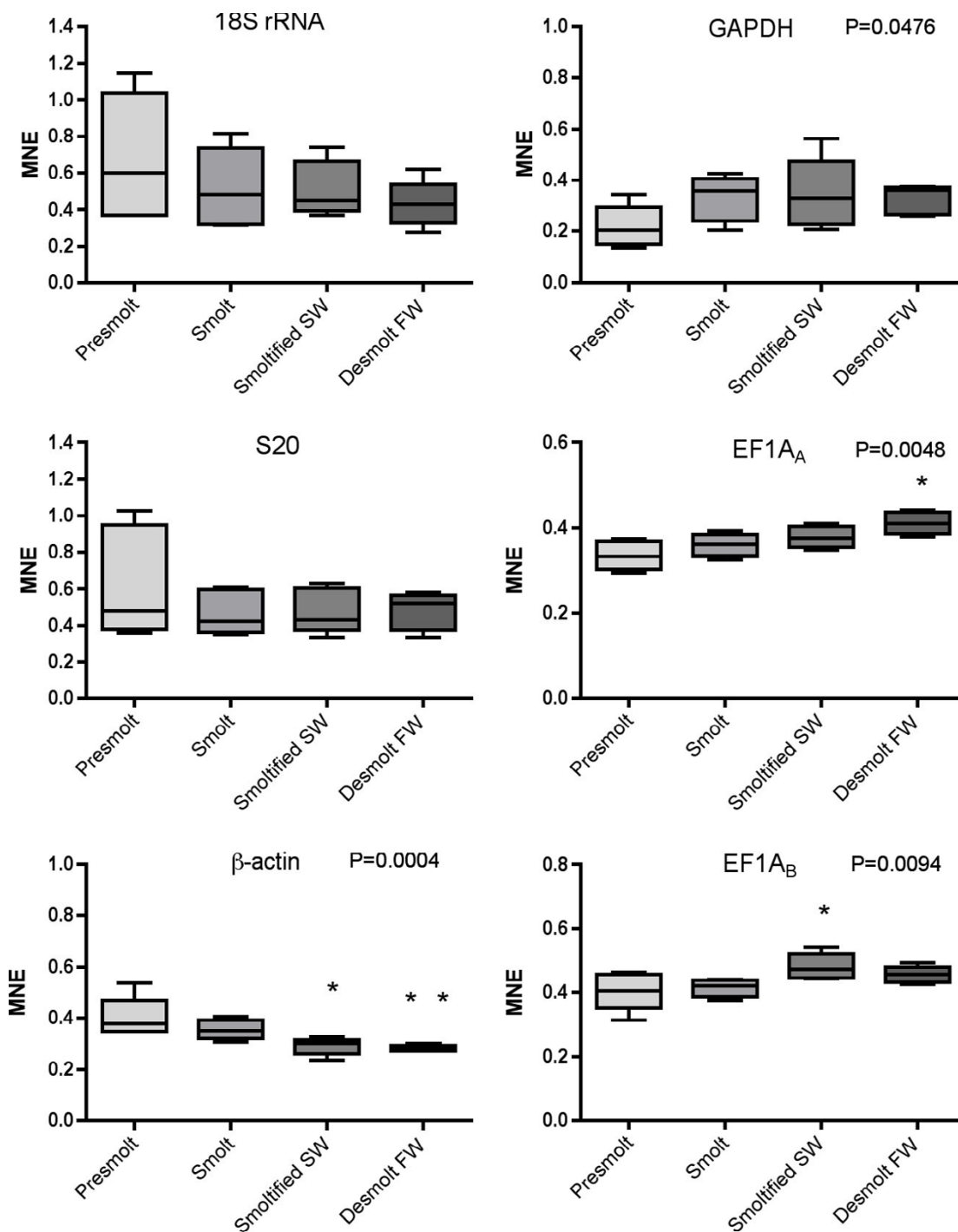
Figure 2 qRT-PCR analysis of six genes in gills of six smoltifying Atlantic salmon. The same data as in Figure 1, but now normalized against an index of the three best genes ( \beta -actin, EF1A A and EF1A B ) calculated with the geNorm software. The four groups were analyzed with Kruskal-Wallis test, and if significant, the overall p-value is given in the graphs. For \beta -actin, there were significant differences between the presmolt and the smoltified group ( p < 0.05 ), the presmolt and the desmolt groups ( n < 0.01 ) and between the smolt and desmolt groups ( p < 0.05 ). For EF1A A , there was a significant difference between the presmolt and the desmolt groups ( p < 0.01 ). For EF1A B , there was a significant difference between the smolt and the smoltified groups ( p < 0.05 ). An asterisk denotes significant differences between the groups.
