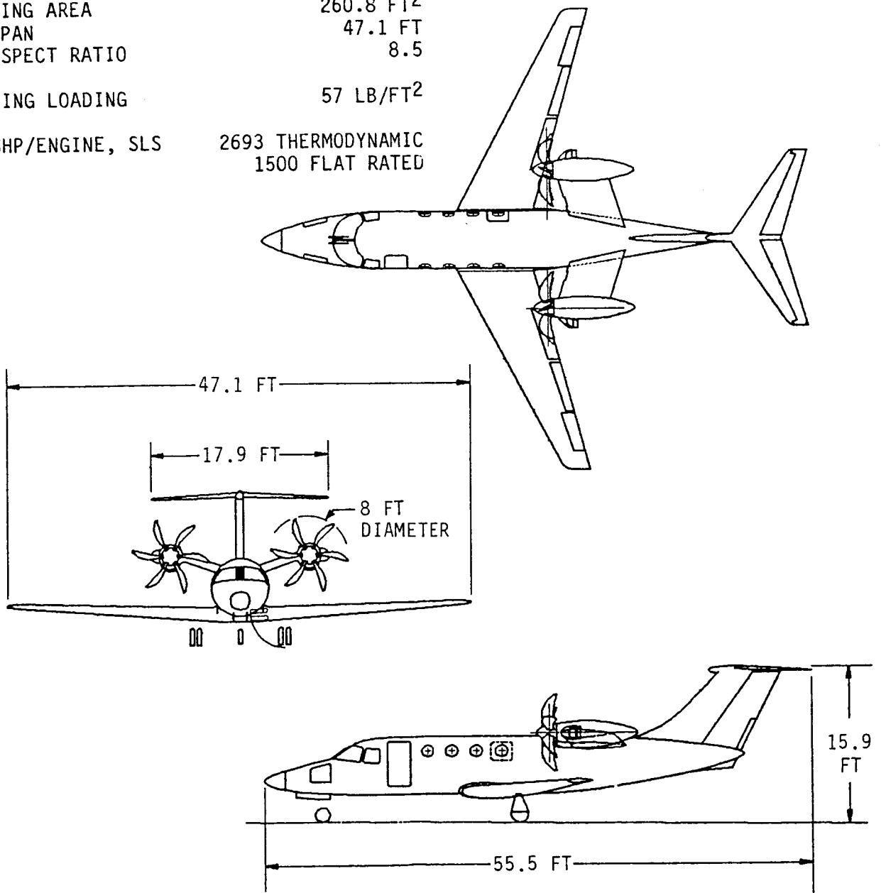
FIGURE 32. 1990 Tractor Propfan Aircraft
