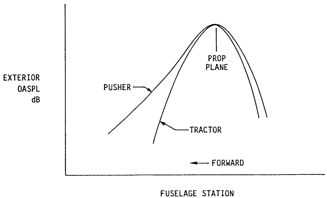
FIGURE 52. Uncertainty in Noise Directivity
