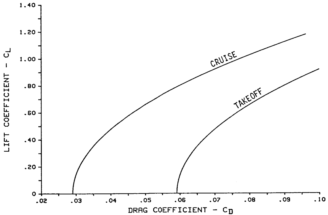
FIGURE 39. Pusher Propfan Low Speed Drag Characteristics
