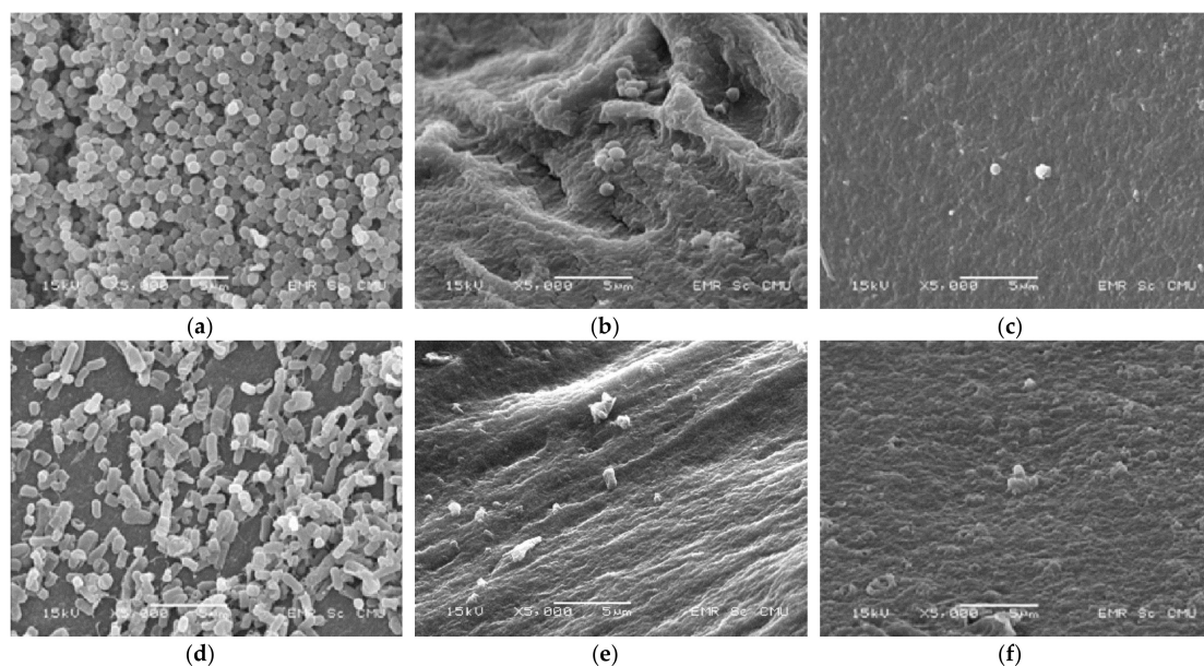
Figure 5. SEM micrographs of untreated S. aureus (a), CTP-treated S. aureus (b), S. aureus treated with PEF at 40 \text{ kV cm}^{-1} and 40 pulses (c), untreated E. coli (d), CTP-treated E. coli (e) and E. coli treated with PEF at 40 \text{ kV cm}^{-1} and 40 pulses (f).
