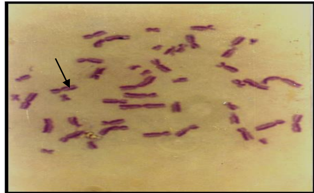
Figure, 1: Microphotographs of sister chromatid exchanges in metaphase chromosomes by fluorescent plus Giemsa staining (1000X).
