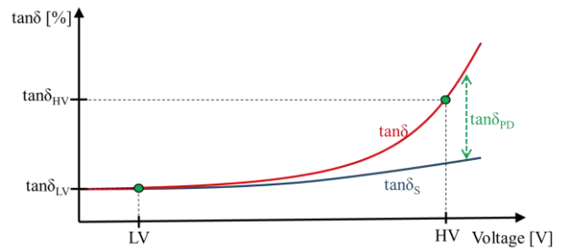
Fig. 2. Test voltage influence on the \tan\delta measurement.
