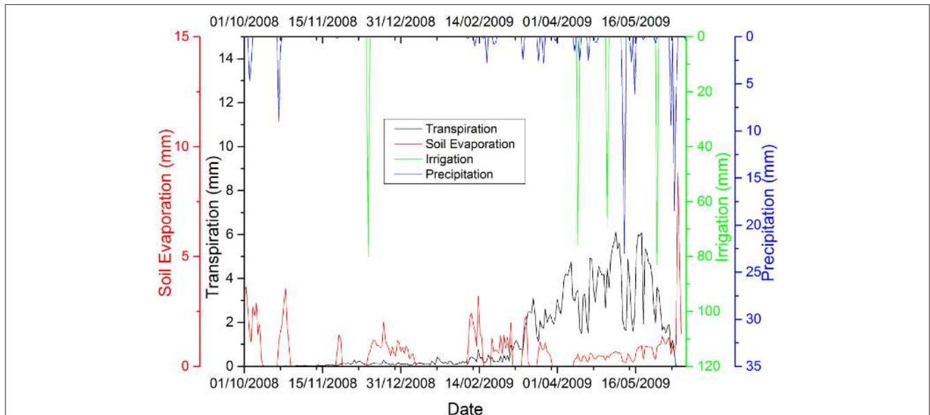
FIGURE 3 | Total daily rainfall (including irrigation) and evapotranspiration partition during the winter wheat growing season of 2008–2009.
