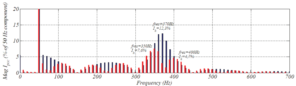
Fig. 22. Harmonic currents at the PCC: With 2 feeders F1-F2 (red) and with 2 feeders on each primary winding F1-F2 and F1'-F2' (black)
