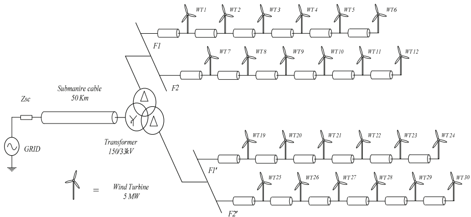
Fig. 21. Simplified scheme of the simulation scenario of the offshore wind farm with two primary windings
