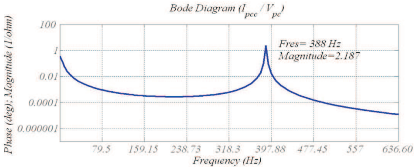
Fig. 14. Frequency response of the transmission system with the cable modeled as 10 “π” circuits in series using state equations
