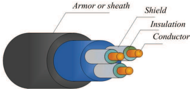
Fig. 1. Generic representation of an electric power cable
