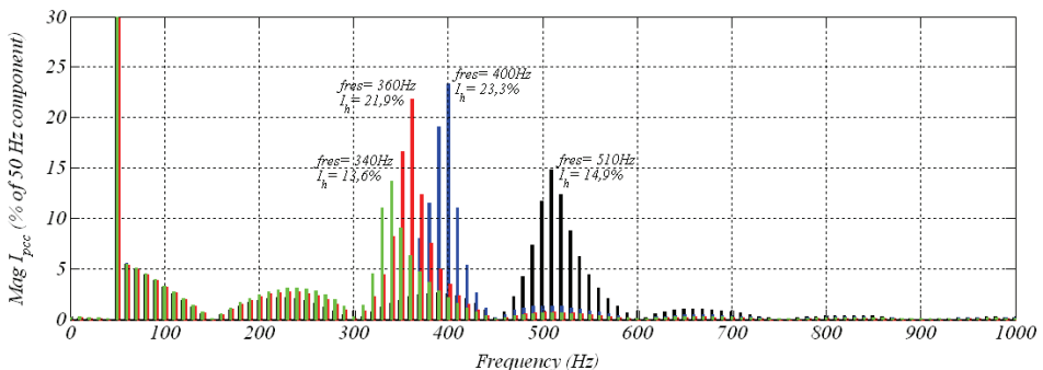
Fig. 11. Frequency response of the transmission system varying the short circuit impedance from: 2 % (black), 5 % (blue), 8 % (green) and 11 % (red)
