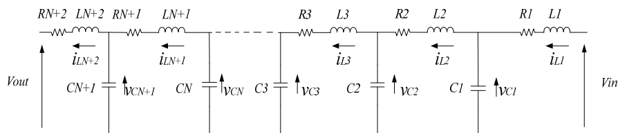
Fig. 13. Mono-phase representation of the transmission system with the submarine cable modeled as N “π” circuits
