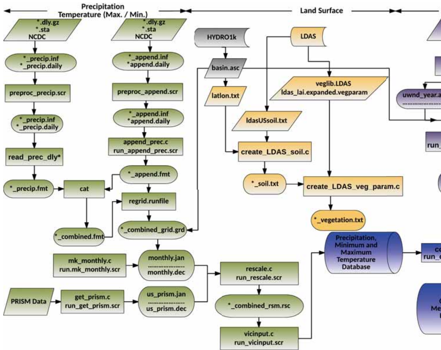
Figure 1. Data pre-processing workflow for the VIC hydrologic model (adapted from Billah et al, 2016).
