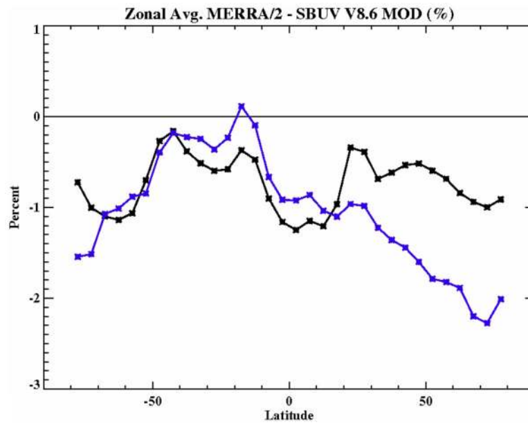
Figure 3. Comparisons of the MERRA-2 total ozone against the Merged Ozone Data Set (MOD). The plot shows the reanalysis minus MOD difference as a percentage of MOD for two periods: 1980–2003 (black) and 2005–2014 (blue).
