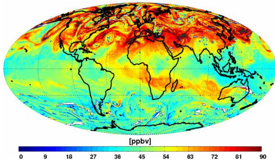
Figure 18. Mean ozone mixing ratio in parts per billion by volume between 500 hPa and the tropopause from MERRA-2 on 1 July 2013. The areas where the tropopause lies below the 500-hPa surface are marked white.
