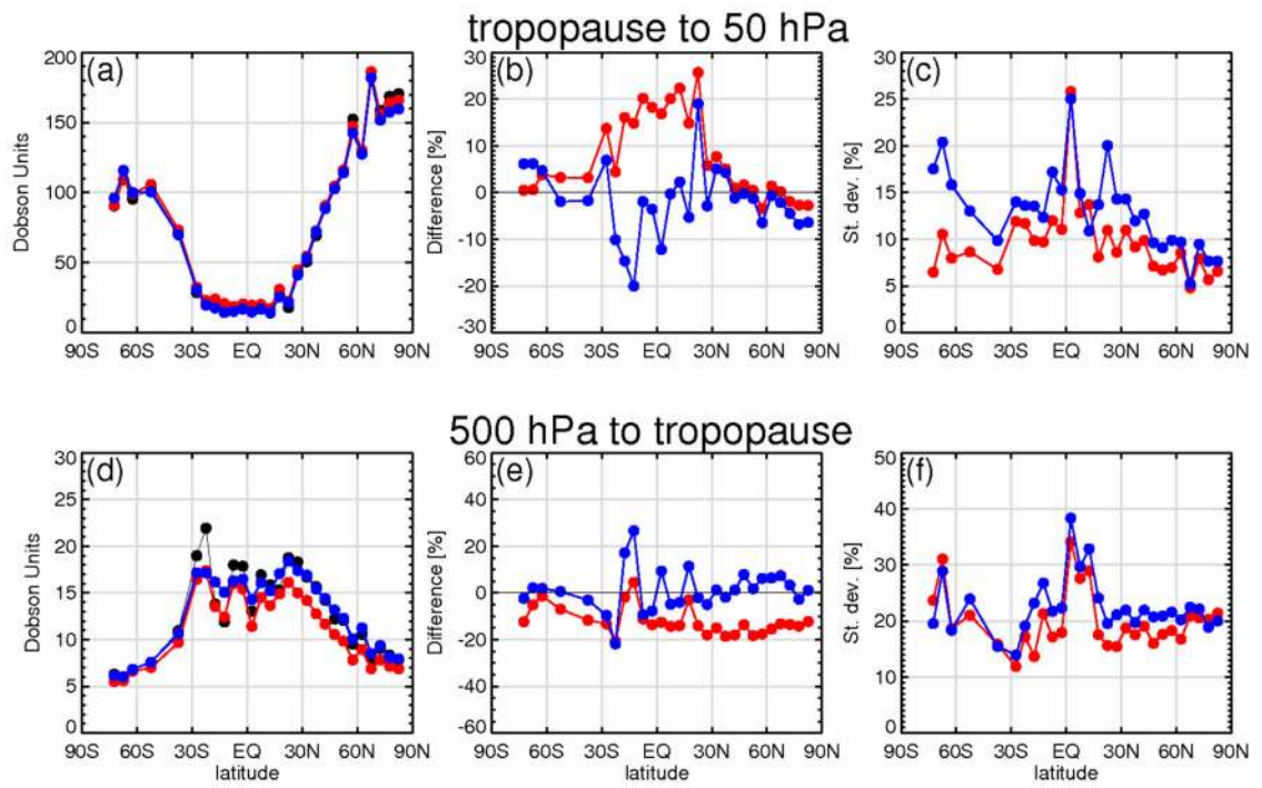
Figure 17. As in Figure 16 but for the 2005–2012 period.
