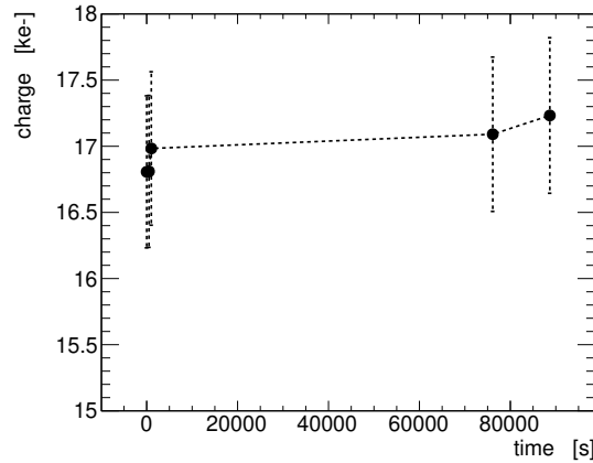
Figure 4: Stability performance. Charge collection vs. time at 1100V of a sample irradiated with protons at 2 \times 10^{15} n_{eq}cm^{-2} .
