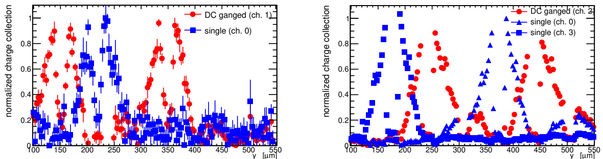
Figure 7: Performance of samples irradiated with protons at 1 \times 10^{15} (left) and 2 \times 10^{15} n_{eq}cm^{-2} (right), with small pitch, DC ganged. Normalized charge collection profile.
