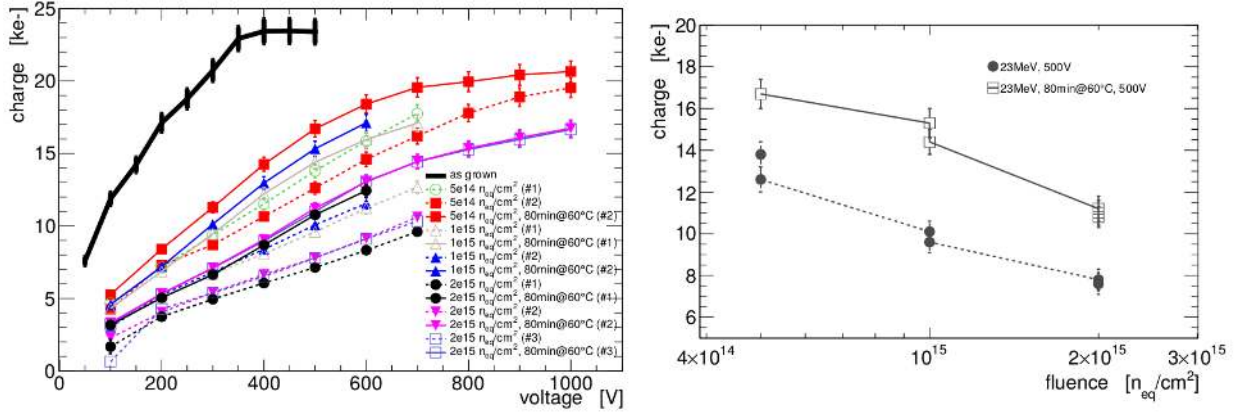
Figure 3: Charge collection vs. bias voltage (left) and vs. fluence (right) of proton-irradiated samples. More sensors per fluence were tested (sensor index in brackets).
