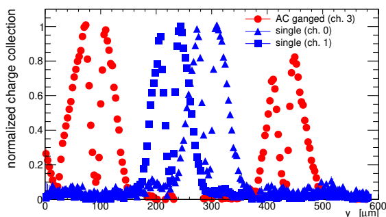
Figure 8: Performance of a sample irradiated with protons at 2 \times 10^{15} n_{eq}cm^{-2} , with small pitch, AC ganged. Normalized charge collection profile.
