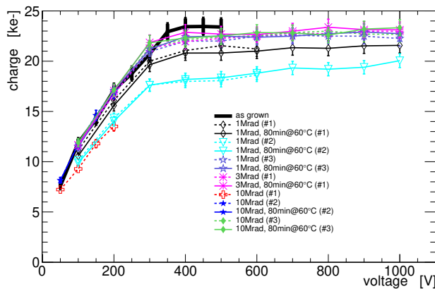
Figure 2: Charge collection versus voltage of \gamma -irradiated samples. More sensors per fluence were tested (sensor index in brackets).
