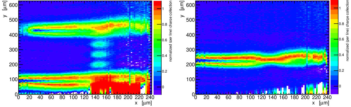
Figure 5: Laser measurements. Normalized charge collection maps of a ganged strip channel (left) and a single strip channel (right) of a sample irradiated with protons at 2 \times 10^{15} \text{ n}_{eq}\text{cm}^{-2} , AC ganged.
