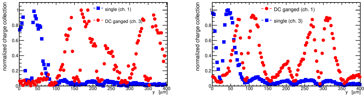
Figure 6: Performance of non-irradiated sample (left) and a sample irradiated at 1\text{Mrad} \gamma -rays dose (right), DC ganged. Normalized charge collection profile.
