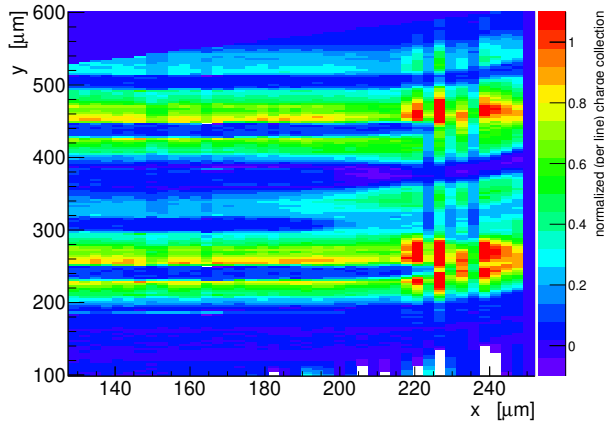
Figure 9: Performance of a sample irradiated with protons at 2 \times 10^{15} n_{eq}cm^{-2} , DC ganged. Normalized charge collection map of a ganged strip channel.
