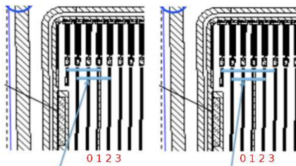
Figure 1: Ganging layout. DC ganging (left) and AC ganging (right) implemented on the miniature sensor under test [9]. The two left most strips, orphans, are connected to neighbours as indicated by the arrows and the horizontal segments; DC ganging connect the orphan metal to the neighbour implant, while AC ganging connect the orphan metal to the neighbour metal.
