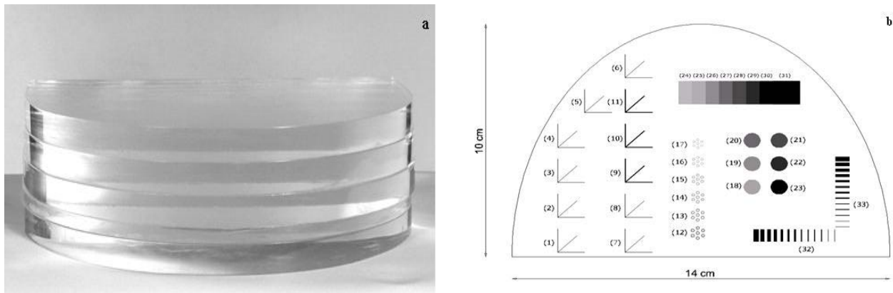
Figure 1. a) A photograph of a constructed phantom. It is consisted from five 10mm thick pieces of D shaped Perspex each with 14cm diameter. b) Phantom structure and components. It is a 0.7cm thickness of parathion containing several components for contrast and spatial resolution in different directions.
