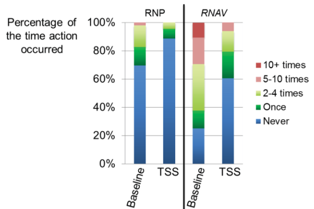
Figure 12. Frequency of path stretch maneuvers for 'New' controllers.
