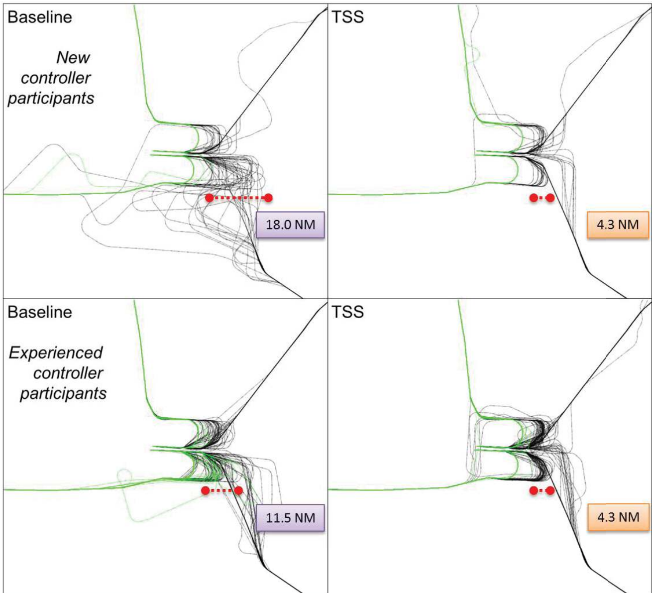
Figure 7. Lateral paths of RNAV/RNP-equipped jets for both sets of controller participants.
