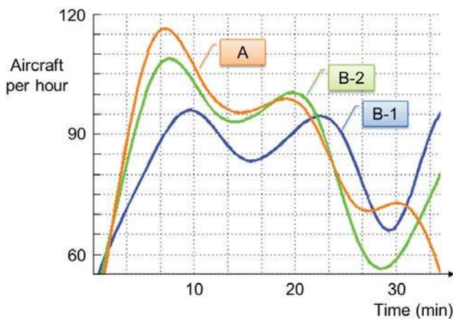
Figure 3. Initial demand rate at the runways.
