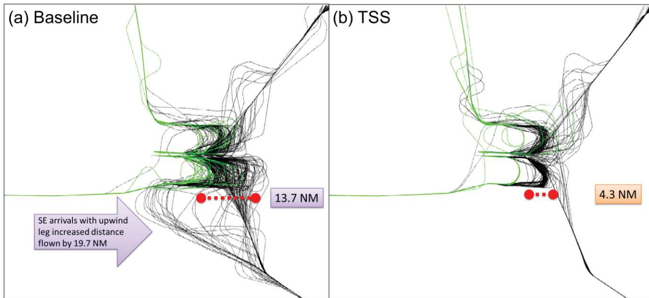
Figure 4. Lateral paths of RNAV/RNP-equipped jets in the (a) baseline case and (b) when using TSS.
