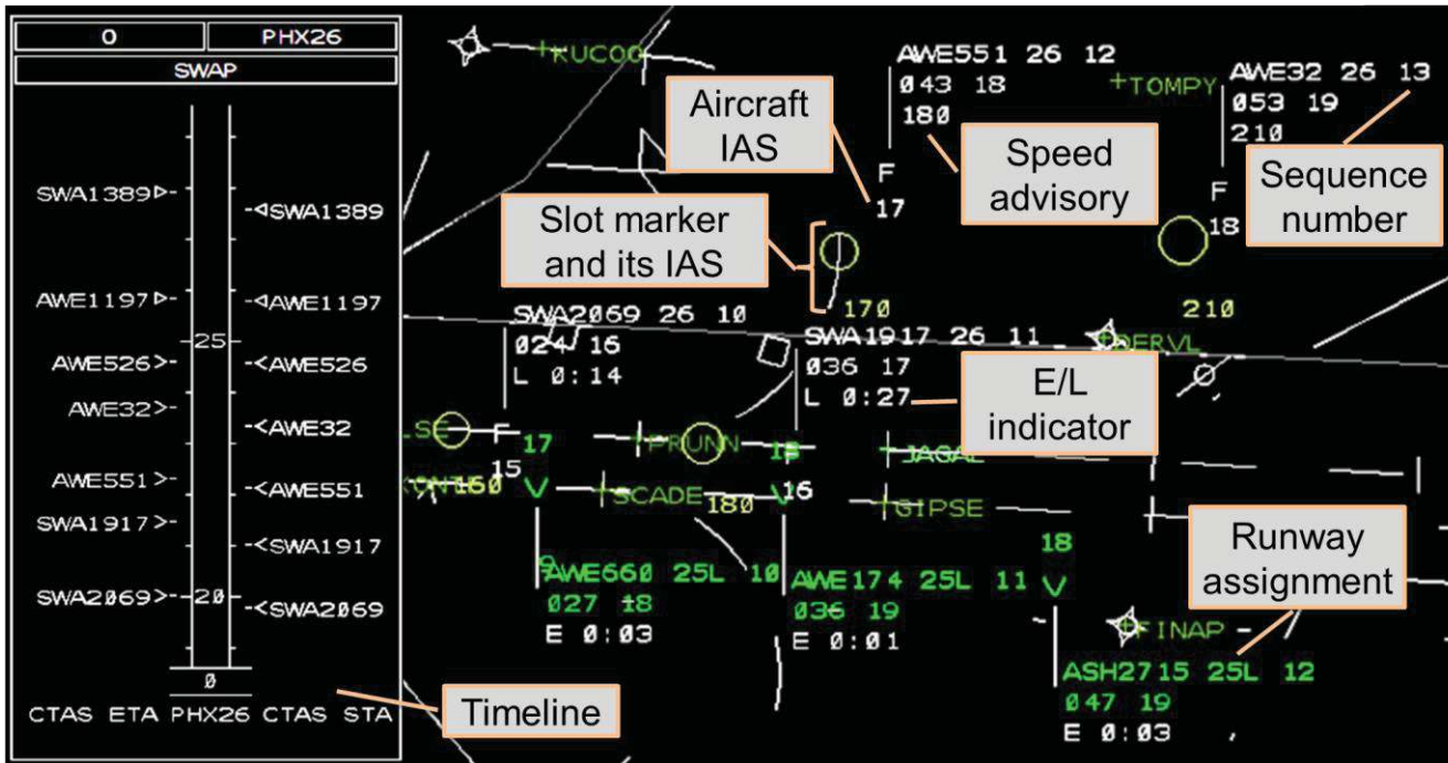
Figure 1. Controller-Managed Spacing toolset.
