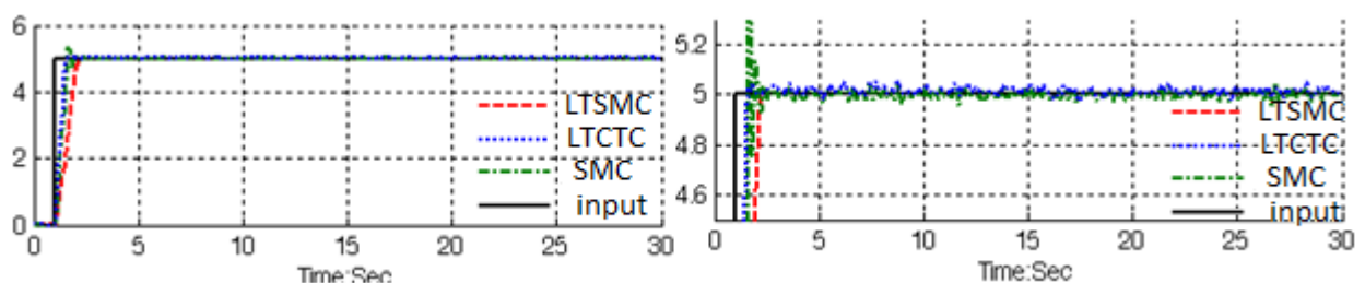
Fig. 6: Desired input, LTSMC, LTCTC and PD-SMC for IC engine trajectory with 20%external disturbance
