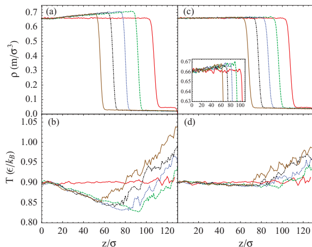
FIG. 6. Density [(a) and (c)] and temperature [(b) and (d)] for a LJ monomer fluid at T_b = 0.9\epsilon/k_B evaporating at a rate j_E = 1.0 \times 10^{-3} \tau^{-1} \sigma^{-2} [(a) and (b)] or j_E = 2.5 \times 10^{-4} \tau^{-1} \sigma^{-2} [(c) and (d)]. From right to left the profiles are plotted every 8000\tau [(a) and (b)] or 24000\tau [(c) and (d)] since the evaporation process was started at t = 0 (the rightmost curve). The inset in (c) shows a blowup of the density in the liquid and interfacial region.
