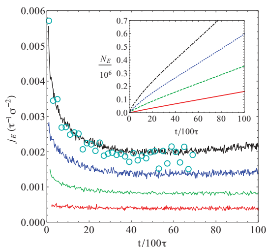
FIG. 8. Evaporation rate j_E vs. time for the LJ dimer system in contact with a vacuum at T_b = 0.9, 1.0, 1.1 , and 1.2\epsilon/k_B (from bottom to top). The predicted evaporation flux j_m/m based on Eq. (9) is shown as circles. The inset shows the total number of removed atoms N_E vs. time.
