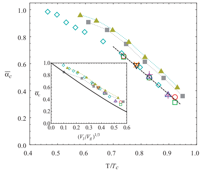
FIG. 15. Condensation coefficient \bar{\alpha}_c vs. temperature for monomers, dimers, and trimers under various evaporation conditions. For monomers: circles ( \circ ) and triangles ( \Delta and \nabla ) are measured using \alpha_c(v_z) ; open squares ( \square ), pluses ( + ), and crosses ( \times ) are measured using p_e(v_z) and p_r(v_z) ; circles ( \circ ) and open squares ( \square ) are for liquid/vapor equilibrium systems at T_i = T_b = 0.8\epsilon/k_B , 0.9\epsilon/k_B , and 1.0\epsilon/k_B ; upward triangles ( \Delta ) and pluses ( + ) are for evaporation rate j_E = 2.5 \times 10^{-4} \tau^{-1} \sigma^{-2} at T_b = 0.9\epsilon/k_B and 1.0\epsilon/k_B ; downward triangles ( \nabla ) and crosses ( \times ) are for evaporation rate j_E = 1.0 \times 10^{-3} \tau^{-1} \sigma^{-2} at T_b = 0.9\epsilon/k_B . For data measured during evaporation, the actual temperature T_i of the liquid/vapor interface is used. The data for dimers and trimers are shown with solid squares ( \blacksquare ) and solid triangles ( \blacktriangle ), respectively, and both are calculated using \alpha_c(v_z) from liquid/vapor equilibrium systems. The dashed line is a linear fit to the monomer data at high temperature. The dotted lines are guides to the eye. Our data of LJ monomers agree with those from Ref. 38 [shown with open diamonds ( \diamond )], which were determined by directly measuring the evaporation flux into a vacuum. The inset plots \bar{\alpha}_c as a function of the translational length ratio, (V_l/V_g)^{1/3} , between the vapor and liquid phase. The solid line in the inset is the prediction of the transition state theory (see Ref. 31).
