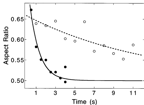
FIG. 1. Thermal relaxation of an atom cloud after one-dimensional heating. The figure shows the time variation of the aspect ratio of the cloud for two different initial densities (solid circles: 5 \times 10^{10} cm -3 ; open circles: 4 \times 10^9 cm -3 ). The lines represent simple exponential fits with time constants of 1.0 and 13 s, respectively.
