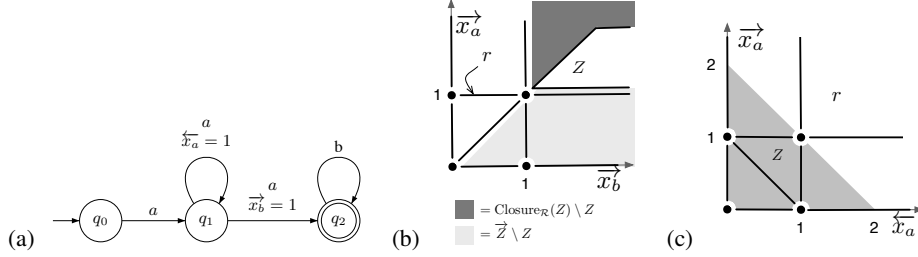
Fig. 3. (a): An ECA for which backward analysis does not terminate. (b) and (c): Examples for \text{Closure}_{\mathcal{R}} and \text{Approx}_k
