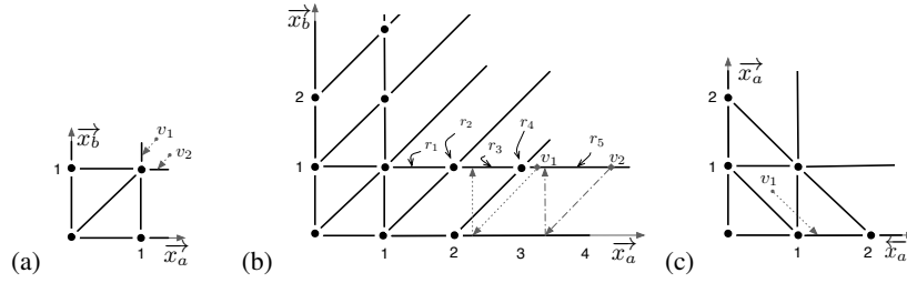
Fig. 2. The sets of regions (a) \text{Reg}(\mathbb{P}_{\{a,b\}}, 1) , (b) \text{Reg}^{\leftarrow}(\mathbb{P}_{\{a,b\}}, 1) and (c) \text{Reg}^{\leftarrow}(\mathbb{C}_{\{a\}}, 1) . Dotted arrows show the trajectories followed by the valuations with time elapsing. Curved arrows are used to refer to selected regions.
