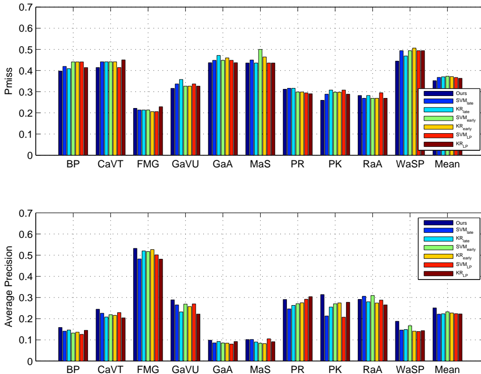
Figure 5. Performance comparison of different algorithms on three features. Full event names of the 10 events can be referred in Section 4.1. LOWER Pmiss values indicate BETTER performance. HIGHER AP values indicate BETTER performance.
