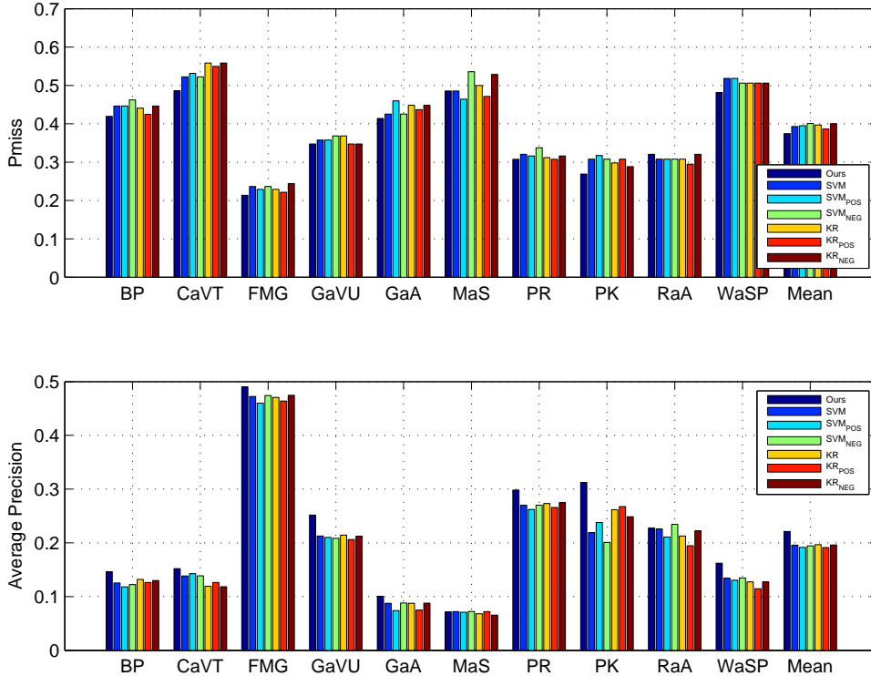
Figure 4. Performance comparison of different algorithms on the single feature Dense Trajectories. Full event names of the 10 events can be referred in Section 4.1. LOWER Pmiss values indicate BETTER performance. HIGHER AP values indicate BETTER performance.
