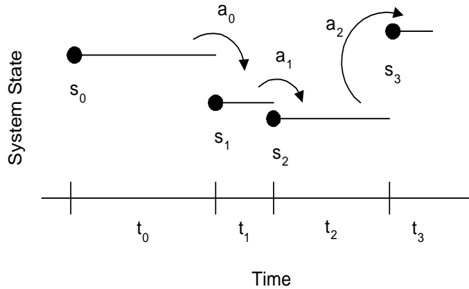
Fig. 10. SMDP Progression
