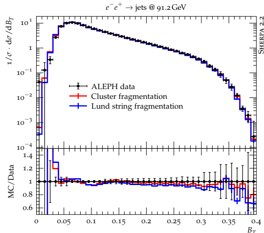
Figure 14: Results for the distribution of the total jet broadening at LEP for the two fragmentation models available in SHERPA in comparison with ALEPH data [193].
