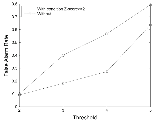
Fig. 8 Effect of condition z -score \geq 2 on false alarm rate
