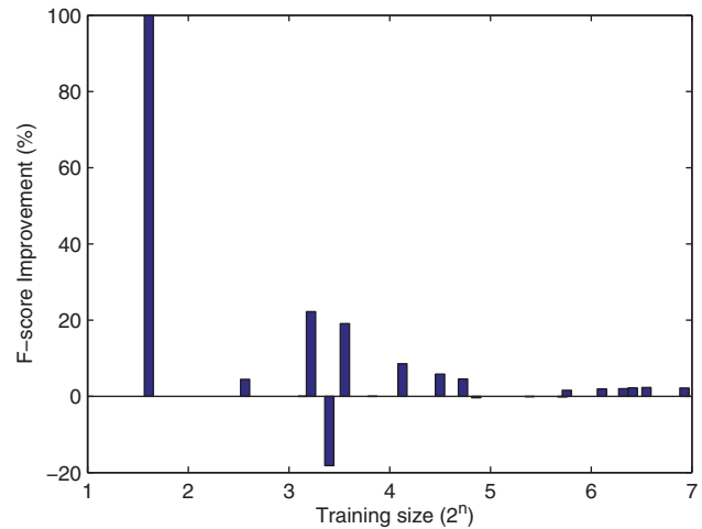
Fig. 2. Performance improvement versus size of training data in each event category
