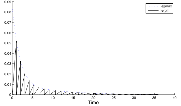
Fig. 2. Evolution of the error norm in the centralized case. The solid line represents the evolution of the error norm \|e(t)\| , which stays below the specified state-dependent threshold \|e\|_{max} = \sigma \frac{\|Lx\|}{\|L\|} which is represented by the dotted line in the Figure.
