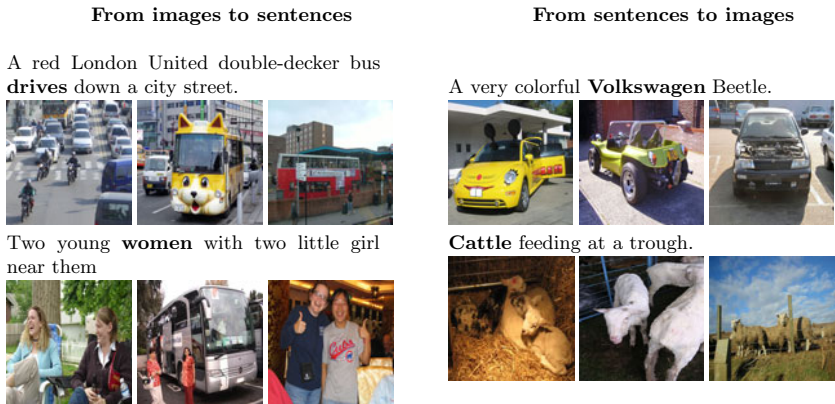
Fig. 6. Out of vocabulary extension: We don't have detectors for "drives", "women", "Volkswagen", and "Cattle". Despite this fact, we could recognize these objects/actions. Distributional semantics provide us with the ability to model unknown objects/actions/categories with their similarities to known categories. Here we show examples of sentences and images when we could recognize these unknowns for both generating sentences from images and finding images for sentences.
