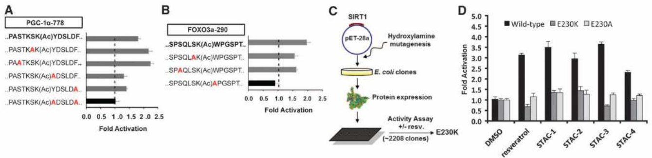
Fig. 2. Substrate sequence requirements and regions on SIRT1 necessary for activation. ( A and B ) SIRT1 activation by STAC-2 on peptides derived from PGC-1 \square -K778 ( A ) and FOXO3a-K290 ( B ) as measured by PNC1-OPT assay; data are means \pm SEM ( n = 3 ). ( C ) Biochemical screen for activation-compromised mutants. A bacterial expression plasmid (pET28a) carrying the SIRT1 gene was mutagenized and used to generate recombinant SIRT1 proteins that were screened for activity in the presence or absence of resveratrol using an AMC-based assay. ( D ) Activation of wild-type SIRT1, E230K, and E230A mutants by 40 \mu M resveratrol, 50 \mu M STAC-1, 5 \mu M STAC-2, 5 \mu M STAC-3, and 10 \mu M STAC-4 as measured by an AMC assay; data are means \pm SD ( n = 3 ). Dimethyl sulfoxide (DMSO) was used as a control.
