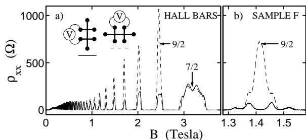
FIG. 4. (a) Anisotropy of \rho_{xx} at T = 25 mK measured using Hall bar samples B (dashed line) and C (solid line). (b) Anisotropy of \rho_{xx} at T = 15 mK measured in the low density sample F . Current flow configurations as in Fig. 3.
