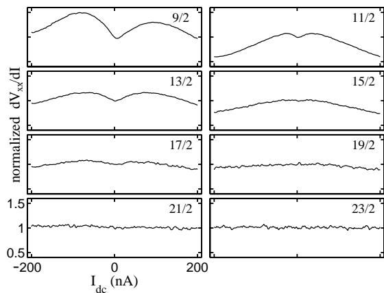
FIG. 5. Nonlinearity of differential resistivity dV_{xx}/dI in sample C at half filling of several high LLs at T = 25 mK. The resistivity is normalized by its value at I_{dc} = 0 . In each panel I_{dc} runs from -200 to +200 nA and the normalized dV_{xx}/dI from 0.5 to 1.5.
