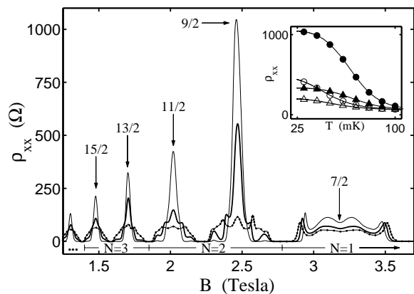
FIG. 2. Peaks in \rho_{xx} in sample A developing at low temperatures in high LLs (dotted line: T = 100 mK; thick line: 65 mK; thin line: 25 mK). Inset: temperature dependence of peak height at \nu = 9/2 (closed circles), 11/2 (open circles), 13/2 (closed triangles), and 15/2 (open triangles).
