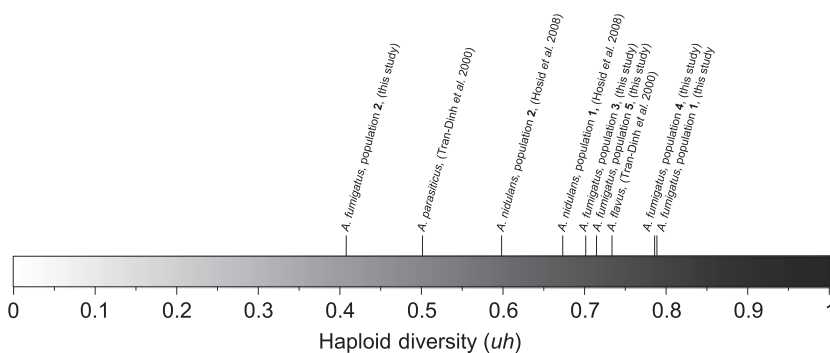
Fig. 3 Unbiased haploid diversity ( uh ) measures of the five Aspergillus fumigatus populations and other representative Aspergillus species. Microsatellite-based uh values from populations of other representative Aspergillus species are from the following studies: A. flavus (Tran-Dinh & Carter 2000), A. parasiticus (Tran-Dinh & Carter 2000) and two A. nidulans populations (Hosid et al. 2008).
