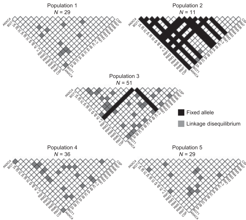
Fig. 4 Linkage disequilibrium (LD) patterns of the five Aspergillus fumigatus populations. The LD patterns of the five A. fumigatus populations. LD was determined by calculating the index of association ( I_a ) for all locus pairs independently for all populations. White, grey and black boxes represent loci in equilibrium, loci in significant LD and fixed loci, respectively.
