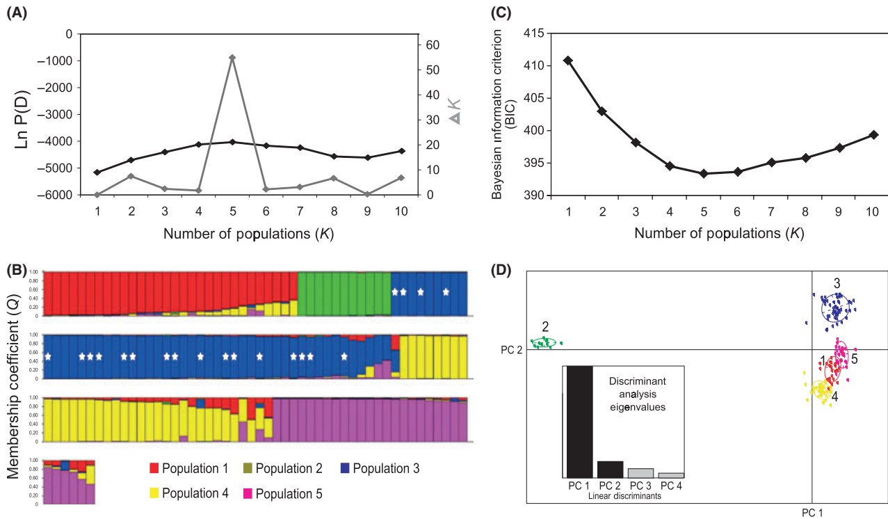
Fig. 2 Both STRUCTURE (panels A and B) and DAPC (panels C and D) analyses of 156 nonclonally related clinical and environmental genotypes identify the existence of five Aspergillus fumigatus populations in the Netherlands. (A) STRUCTURE analysis estimates that the optimal predicted number of populations K for our set of genotypes is five. This inference is supported by both the average log probability ( \text{Ln}P(D) ) of each K value (black line) and by the ad hoc statistic \Delta K (grey line). (B) The STRUCTURE-based assignment of 156 genotypes into the five A. fumigatus populations. Each column on the X-axis corresponds to a different genotype. The Y-axis represents an individual's membership coefficient to each population. White stars indicate multi-triazole-resistant (MTR) individuals. Structure populations 1–5 are indicated by red, green, blue, yellow and pink colour, respectively. (C) DAPC analysis estimates that the optimal predicted number of populations K for our set of genotypes is five. The Y-axis corresponds to the Bayesian information criterion (BIC), a goodness-of-fit measurement calculated for each K . The lowest BIC value ( K = 5 ) indicates the optimal number of populations. (D) DAPC clustering of the five populations using the first two principal components (Y-axis and X-axis, respectively). The first four eigenvalue components are shown in the lower left panel. DAPC populations 1–5 are indicated by red, green, blue, yellow and pink colour, respectively, and are highly similar to STRUCTURE delineated populations.
