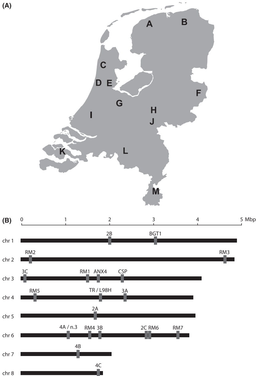
Fig. 1 (A) Sampling location of the 156 genotypes from the Netherlands and (B) the chromosomal location of the TR/L98H (MTR) locus and the 20 markers used in the present study. In panel A, city and number of isolates and genotypes collected per city, respectively (in parentheses), are as follows: A: Leeuwarden (8, 3), B: Groningen (1, 1), C: Alkmaar (10, 9), D: Haarlem (7, 5), E: Amsterdam (19, 10), F: Enschede (15, 9), G: Utrecht (21, 7), H: Arnhem (6, 3), I: Rotterdam (45, 29), J: Nijmegen (102, 68), K: Goes (7, 5), L: Veldhoven (9, 4) and M: Heerlen (5, 3). The chromosome length scale (in million base pairs or Mbp) is shown on top of panel B.
