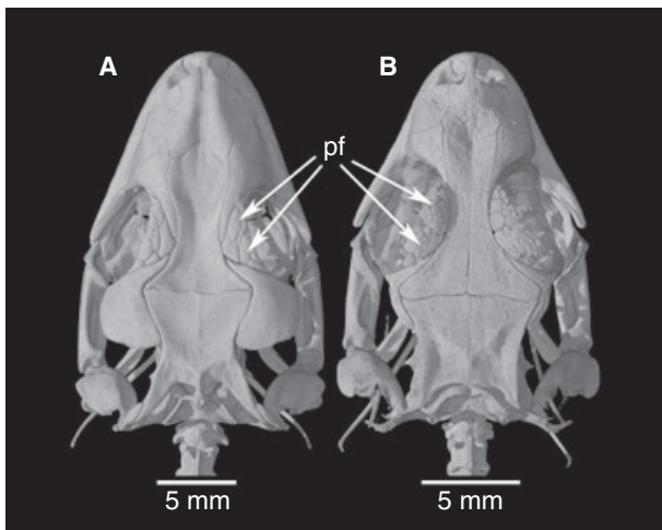
Figure 4 Dorsal views of skulls of (a) Aristelliger georgeensis (CAS 176485); (b) Teratoscincus przewalskii (CAS 171013) showing the position of the parafrontal bones (pf), a putative synapomorphy of the clade subtended by node E (Fig. 3). Skulls were imaged from intact specimens using high-resolution X-ray computed tomography.
