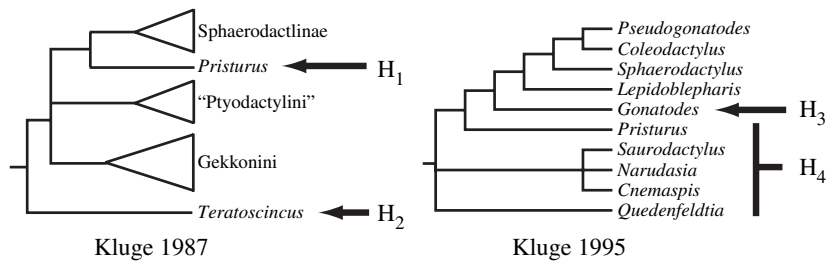
Figure 1 Previous phylogenetic hypotheses of Gekkotan lizards with special emphasis on the Sphaerodactylinae and allied taxa. Modified from Kluge (1987, 1995). Alternative phylogenetic hypotheses tested in this paper are indicated with arrows.
