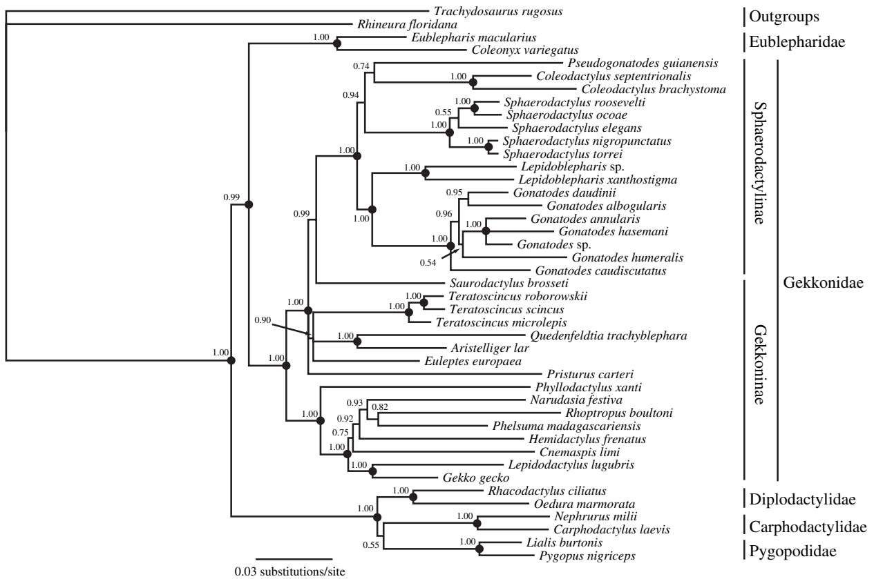
Figure 2 Bayesian phylogram using the best-fit partition strategy, with data partitioned by gene and codon. Labels above nodes represent the posterior probabilities. Black circles indicate nodes with parsimony bootstrap values > 70. Higher-level taxonomy follows Han et al. (2004).
