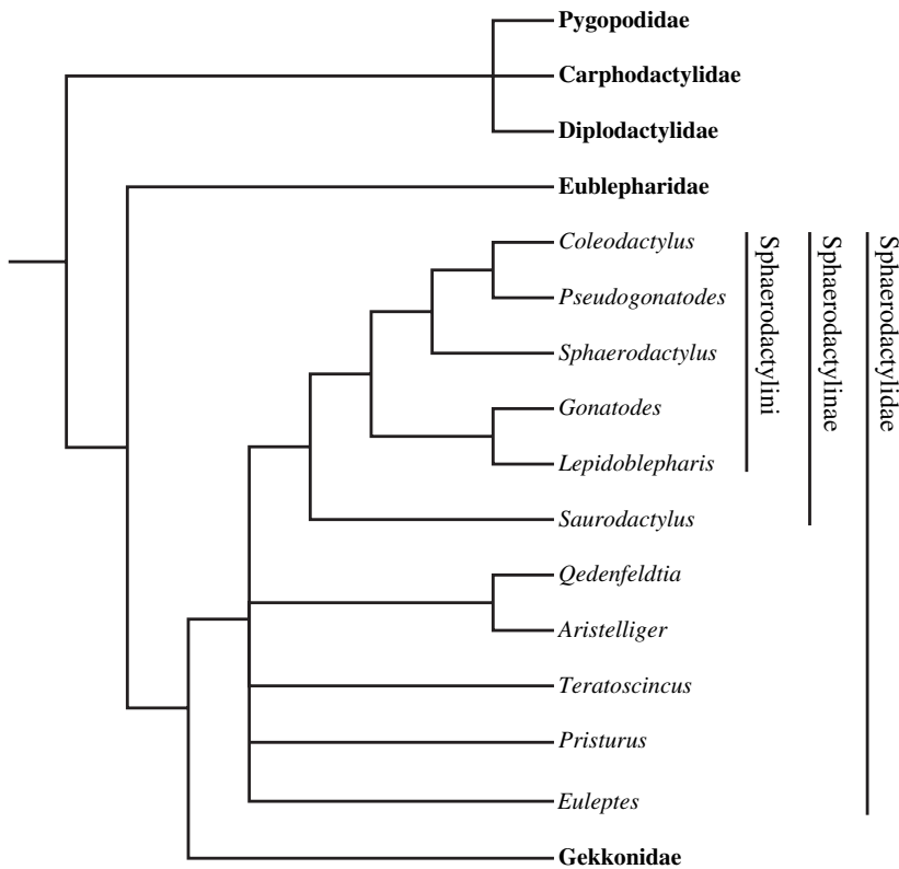
Figure 5 Summary of the phylogenetic relationships and higher level taxonomy of the sphaerodactyl geckos and related genera, as presented in this paper.
