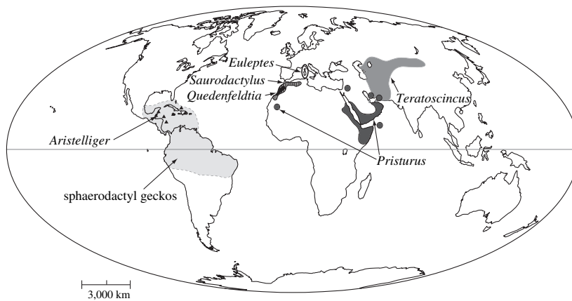
Figure 6 Geographical distributions of the Sphaerodactylidae. The 'sphaerodactyl geckos' include the genera Coleodactylus , Gonatodes , Lepidoblepharis , Pseudogonatodes and Sphaerodactylus . Sources include Aristelliger (Powell et al. , 1996; Köhler, 2003); Euleptes (Bauer et al. , 1997); Pristurus (Geniez & Arnold, 2006); Quedenfeldtia and Saurodactylus (Bons & Geniez, 1996; Schleich et al. , 1996); sphaerodactyl geckos (Kluge, 1995); and Teratoscincus (Macey et al. , 2005). The map uses an equal-area, Mollweide projection.
