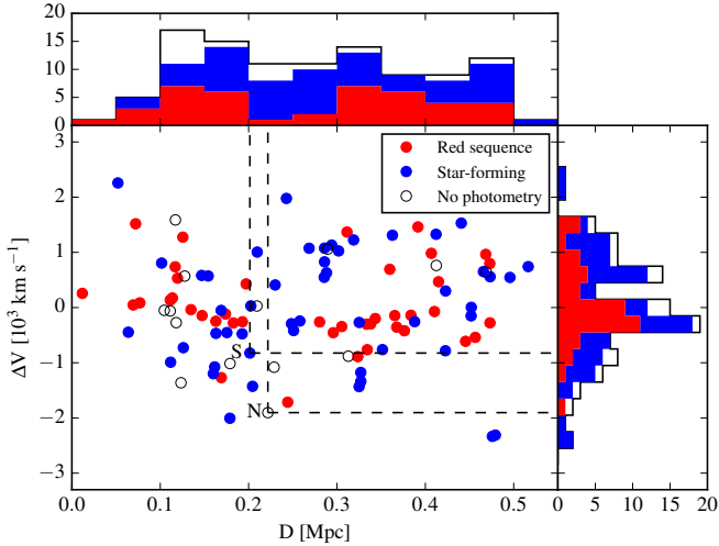
Fig. 2. Phase-space diagram of galaxies in cluster CGr32 determined using the barycentre of the cluster members identified spectroscopically with MUSE as the cluster centre. Quiescent galaxies are indicated with red-filled dots, star-forming objects with blue-filled dots. Black open circles show blended galaxies with unavailable broad-band photometry. The galaxies ID 345 and ID 473 are indicated with “S” and “N”, respectively.
