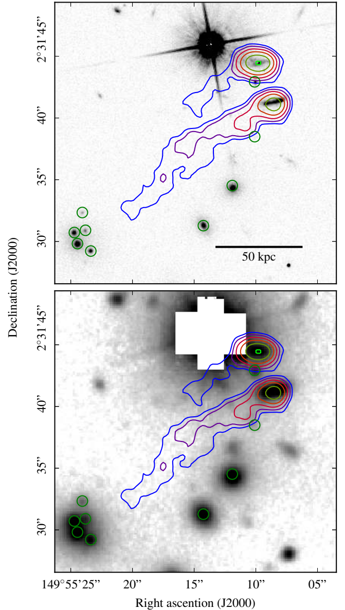
Fig. 3. F814W HST ACS (top) and i -band Suprime-Cam (bottom) images of galaxies ID 345 (south) and ID 473 (north) in cluster CGr32. Other cluster members are shown with green circles. Contours show the [\text{O II}] flux map obtained using a Gaussian smoothing of 3 pixels FWHM at a level of \Sigma([\text{O II}]) = 1.5, 3.3, 7.4, 16.3, 36.1, 80.0 \times 10^{-18} \text{ erg s}^{-1} \text{ cm}^{-2} \text{ arcsec}^{-2} . Both images (oriented as in the sky, north is up, east on the left) show the lack of any optical counterpart along the tail.
