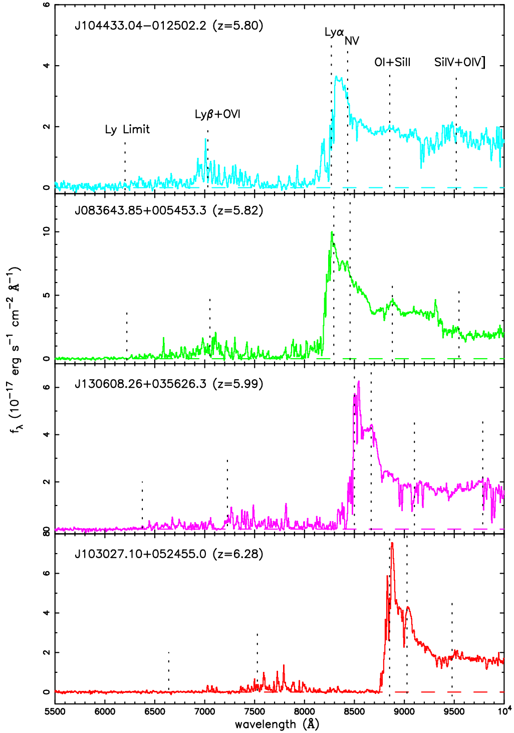
FIG. 1.— Optical spectra of z \gtrsim 5.8 quasars observed with Keck/ESI, in the observed frame. The spectra have been smoothed to 4\text{\AA} \text{pixel}^{-1} , and have been normalized to the observed z band flux. The spectrum of SDSS1044-0125 has been taken from Fan et al. (2000). In each spectrum, the expected wavelengths of prominent emission lines, as well as the Lyman limit, are indicated by the dashed lines.
