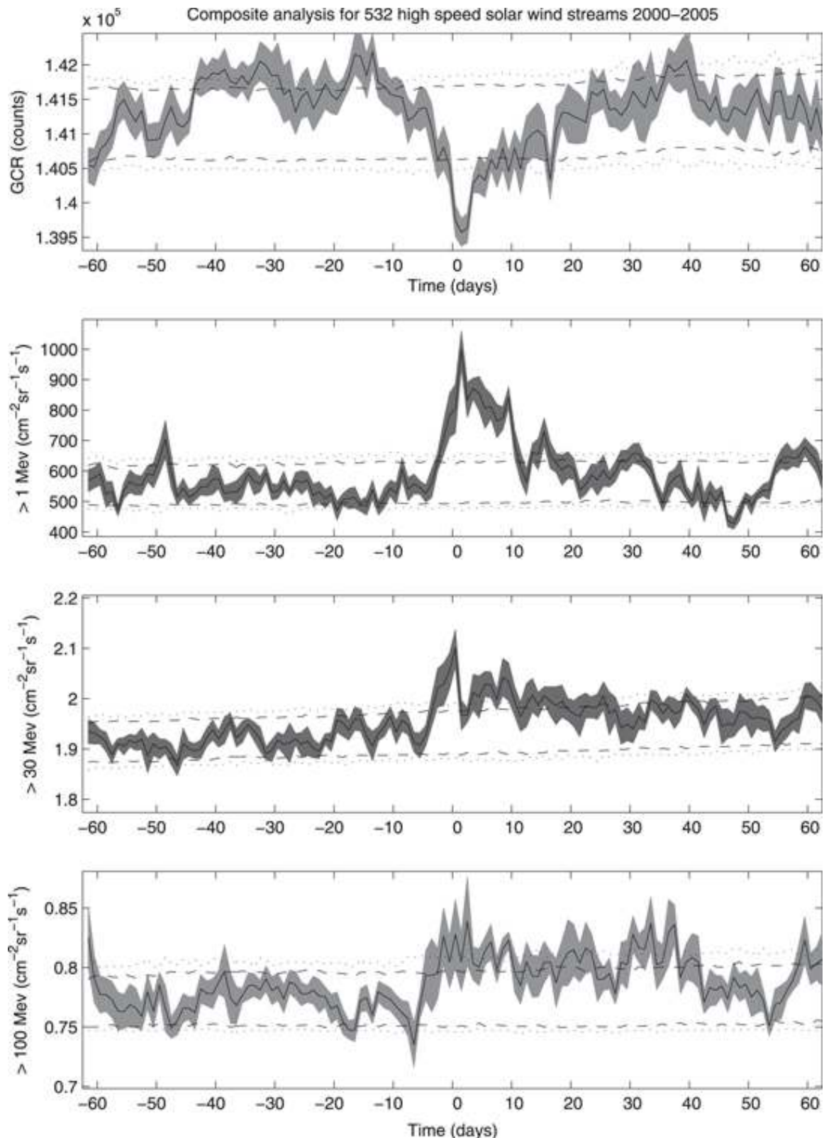
Figure 3. Median response in galactic cosmic ray flux (top panel) as measured by the ground-based neutron monitor at Oulu, Finland. The second, third and fourth panels present median proton flux measurements from the GOES satellite dataset for three energy channels; >1 Mev (top), >30 Mev (middle) and >100 Mev (lower). The median response in each parameter is represented by a solid line, the standard error in this median as a grey area around the line while the dashed lines and the dotted lines correspond to the 95% and 99% levels of the dataset respectively. These percentile levels were calculated by repeating the analysis many times using random trigger times and determining the levels in each time bin that contained 95 and 99% of the data points.
