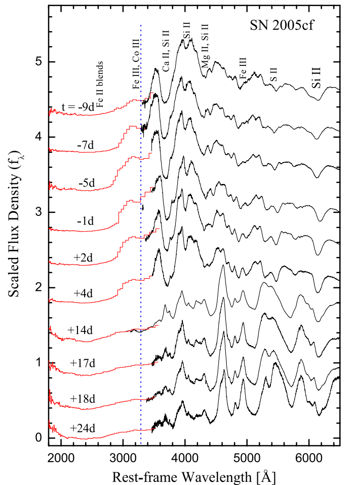
Figure 5. Evolution of the UV–optical spectrum of SN 2005cf. The UV spectra were obtained with the HST ACS prism (PR200L), and the corresponding optical data are taken from W09b and Garavini et al. (2007). All of the spectra have been rescaled to match the UV–optical photometry and were adjusted to the peak of the spectral flux and arbitrarily shifted for display. The dashed line marks the position of the \sim 3250 Å absorption feature. The increase in flux below about 2200 Å is almost certainly an artifact and should not be trusted.
