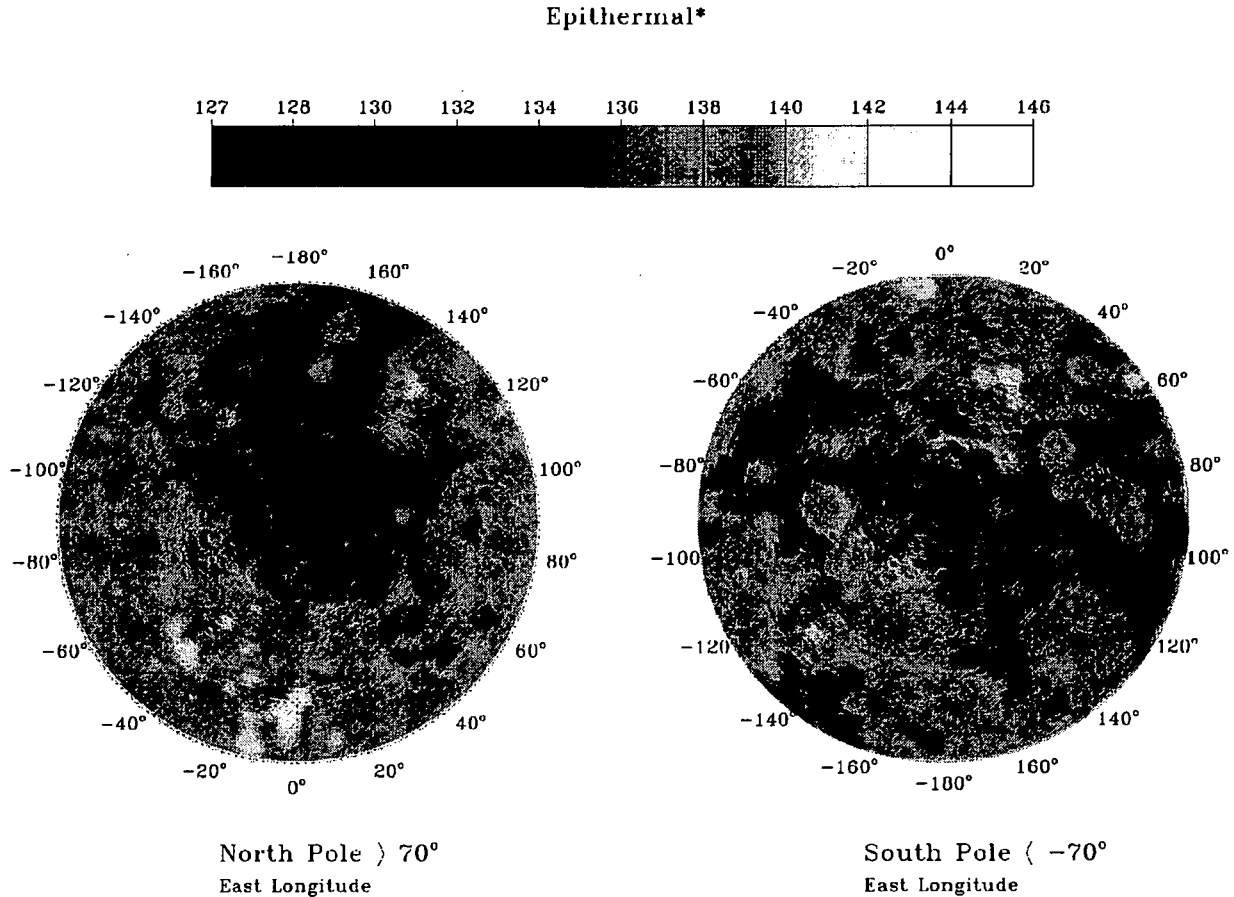
Figure 1. Overlays of stereographic projections of the Epi* neutron flux and Clementine 750 nm intensity poleward of +70° (left) and -70° (right) latitudes.
