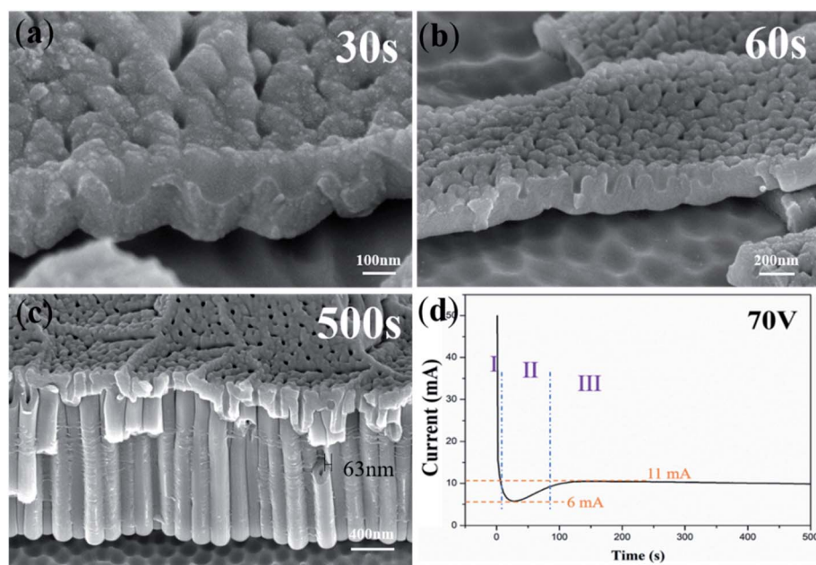
Fig. 1 FESEM images of anodic TiO 2 nanotubes anodized for (a) 30 s; (b) 60 s; (c) 500 s and (d) the corresponding current–time curve.
