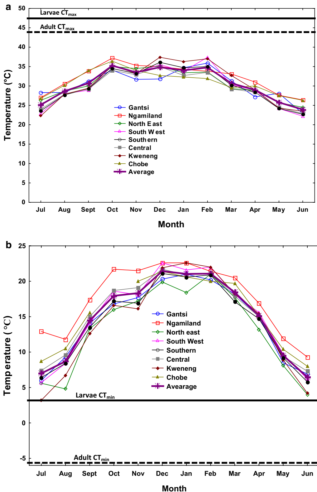
Fig. 4 Field temperatures, a mean monthly maximum temperatures and b mean monthly minimum temperatures for eight districts of Botswana in 2015/16 season related to T. absoluta CT_{max} and CT_{min} , respectively. Horizontal lines denote CT_{min} and CT_{max} for larvae (continuous) and adult (dotted)
