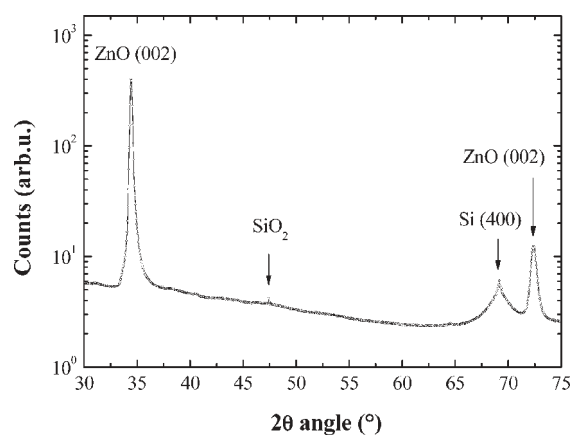
Figure 1. \omega-2\theta (with \omega = \theta - 1^\circ ) XRD pattern of the \text{Zn}_{0.9}\text{Co}_{0.1}\text{O} thin film.
