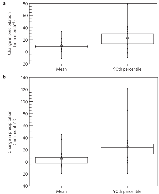
Figure 4 | Projected changes in mean and extreme monthly rainfall in central Tanzania. a, b , Projected changes in precipitation over the period 2070–2099 relative to 1961–1990 for a 10° box centred on the Makutapora Wellfield in central, semi-arid Tanzania from multi-model ensembles of CMIP3 (AR4) under the A1B emissions scenario (23 GCMs) ( a ) and CMIP5 (AR5) under the RCP8.5 scenario (21 GCMs) ( b ). Box plots are of changes in monthly precipitation for each model in the MME. Dots indicate individual models within the MME sample, boxes show the inter-quartile range and median and circles show the mean of the MME sample.
