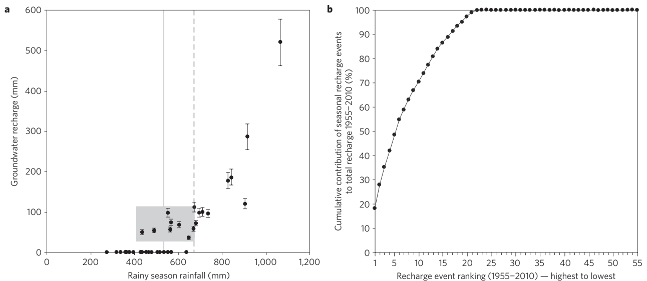
Figure 2 | Analysis of the relationship between groundwater recharge and rainfall. a , Cross plot of observed recharge from groundwater-level fluctuations versus rainy season (November to April) rainfall. b , Cumulative contribution of annual recharge to the total recharge received at the Makutapora Wellfield from 1955 to 2010. The shaded region in a indicates seasons featuring a month of statistically extreme (>95th percentile) rainfall, the solid vertical line in a indicates the median (50th percentile), and the dashed line indicates the third quartile (75th percentile) rainy season rainfall.
