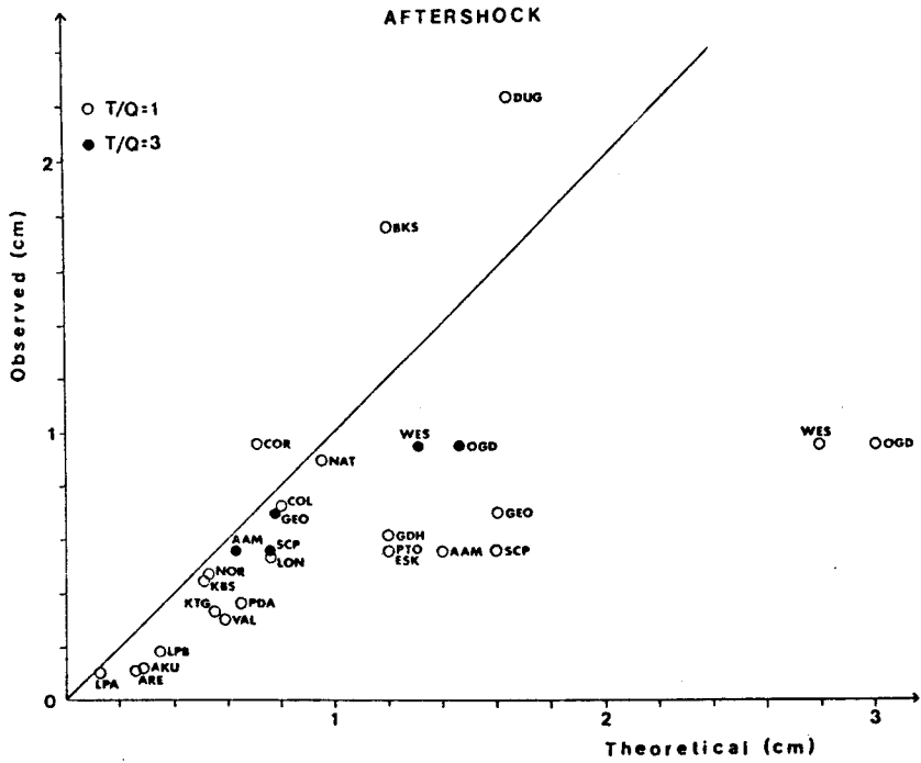
Fig. 4. Comparison of observed and theoretical amplitudes for the aftershock.
