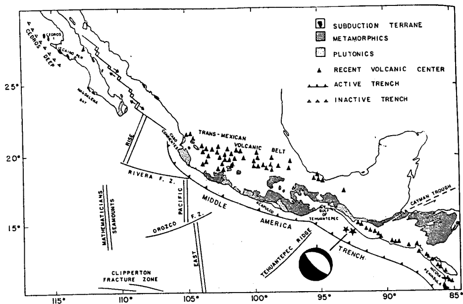
Fig. 1. Map of Mexico and Central America showing plate boundaries and other geological features. Earthquakes selected for study denoted by (*). Epicentral coordinates are given in Table 1. Focal mechanism diagram is also shown. The darkened quadrants are the quadrants of dilatation, first motion. (Base map taken from Karig et al. (1978).
