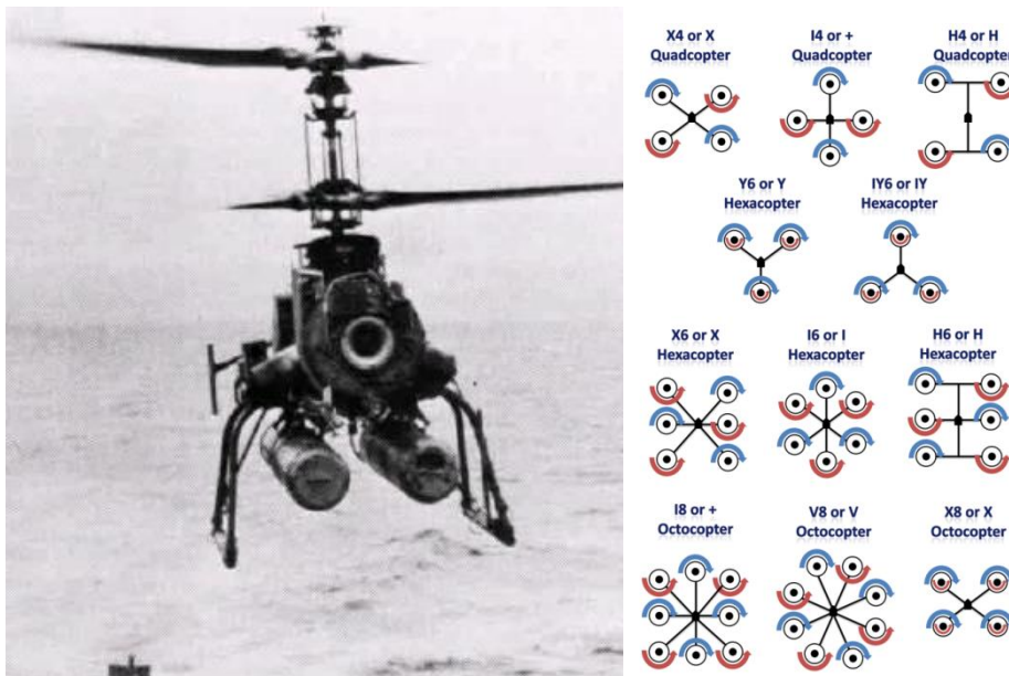
Fig. 9: Left-hand-side, Gyrodyne QH 50 DASH, and right-hand-side, most common rotor configurations in multirotor helicopter UAVs.
