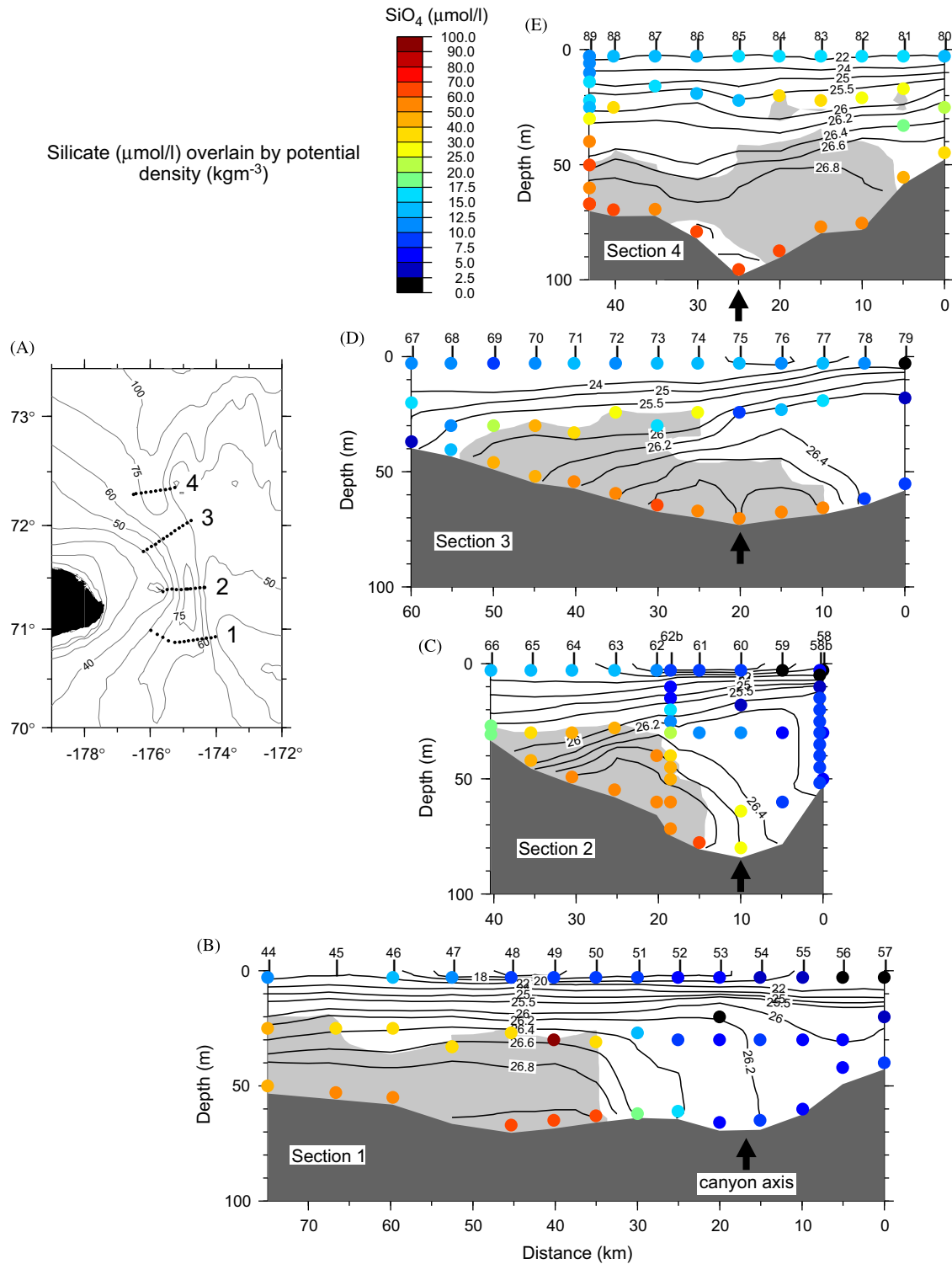
Fig. 5. Evolution of the silicate distribution from south to north in Herald Canyon. The presentation is the same as in Fig. 2. The colored circles in (B)–(E) denote SiO 4 concentration, overlain by potential density (contours). The gray shading denotes the winter water (potential temperature ≤ -1.6 °C). (For interpretation of the references to color in this figure legend, the reader is referred to the web version of this article.)
