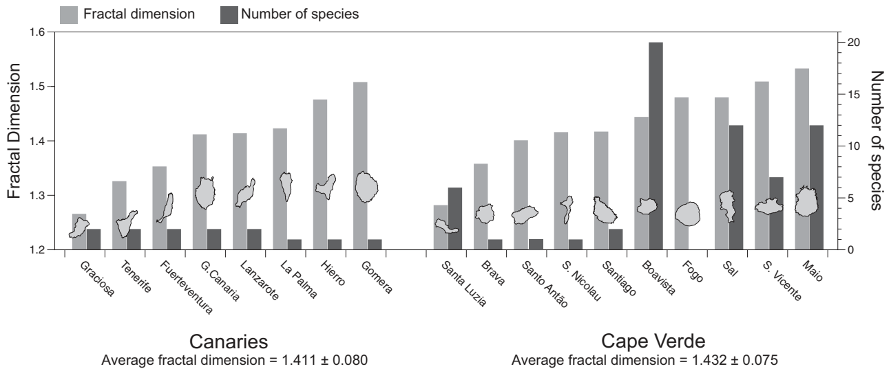
FIGURE 4. Coastline fractal dimension of Cape Verde and Canarian archipelagos using Fractal Dimension Calculator V1.01. Bars represent the fractal dimension of each island (light gray) and the total number of species (dark gray), endemics, and nonendemics. The contour of the coastline of each island is shown.
