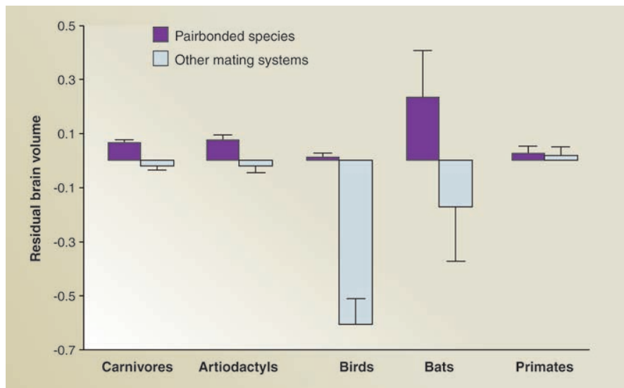
Fig. 3. Mean ( \pm SE) of residual brain volume (controlling for body size and phylogeny) in species with pairbonded (purple bars) versus all other mating systems (gray bars) in birds and four orders of mammals. The differences are significant in all cases except primates.
